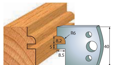
Pair of knives 690.134 Pair of limiters 691.134
