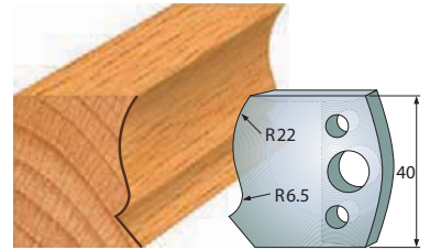
Pair of knives 690.128 Pair of limiters 691.128
