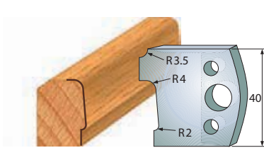
Pair of knives 690.130 Pair of limiters 691.130
