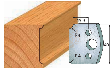
Pair of knives 690.171 Pair of limiters 691.171
