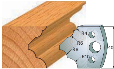
Pair of knives 690.126 Pair of limiters 691.126
