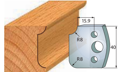
Pair of knives 690.174 Pair of limiters 691.174
