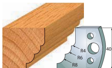
Pair of knives 690.132 Pair of limiters 691.132
