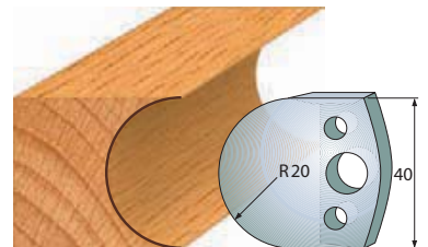
Pair of knives 690.131 Pair of limiters 691.131
