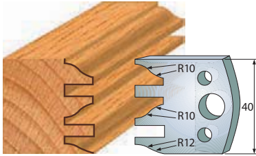
Pair of knives 690.124 Pair of limiters 691.124
