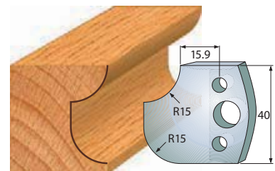
Pair of knives 690.177 Pair of limiters 691.177
