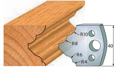
Pair of knives 690.125 Pair of limiters 691.125
