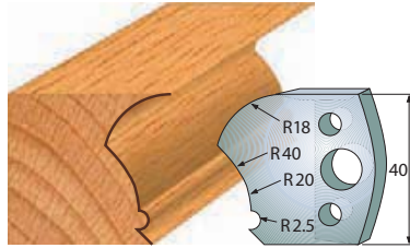
Pair of knives 690.123 Pair of limiters 691.123
