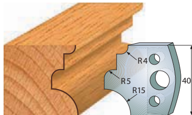
Pair of knives 690.129 Pair of limiters 691.129
